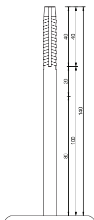
UNI-Flexplug 330080
