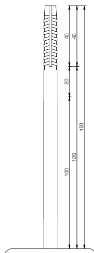
UNI-Flexplug 3300100
