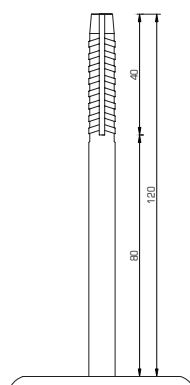
UNI-Flexplug 330065
